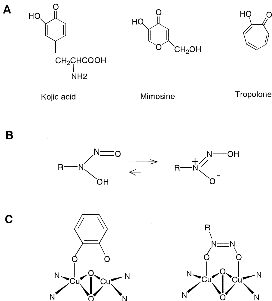
Figure 4. (A) The known potent inhibitors. (B) A possible planar structure of the tautomeric hydroxydiazene N -oxide. (C) Binding models to the binuclear copper active center in the oxy -form of tyrosinase. N -nitrosohydroxylamines (right) may also interact with the binuclear copper as shown for catechol (left, ref 22).
